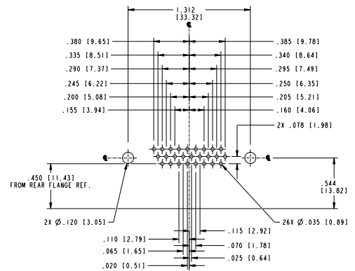
DAMM26S (Receptacle)
